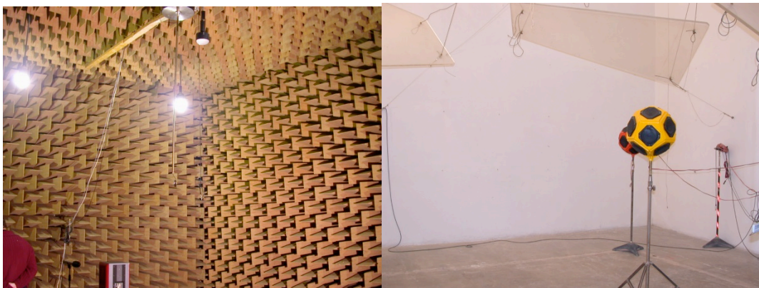
Figure 2. Anechoic (left) and Reverberant (right) Chambers at the ITEFI
